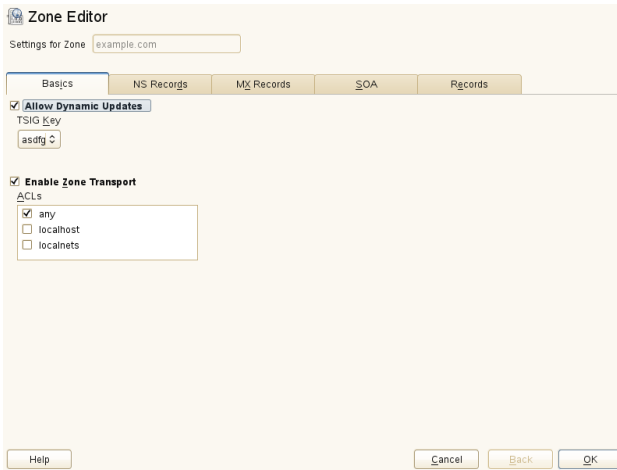
Figure 25.5: DNS Server: Zone Editor (Basics)
