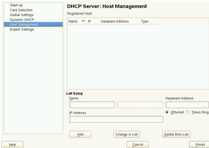
Figure 26.5: DHCP Server: Host Management
