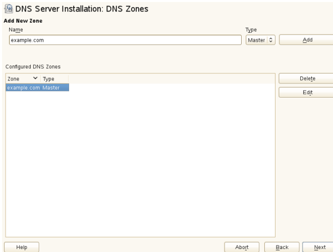
Figure 25.2: DNS Server Installation: DNS Zones
