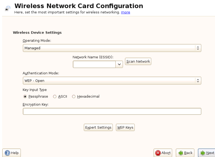
Figure 19.1: YaST: Configuring the Wireless Network Card
